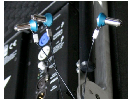
Goupille "K-Pin"
